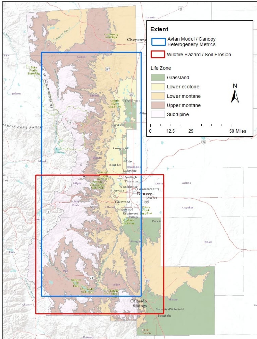
Figure 1. Extent of ecosystem service metrics included in the map package 2018 layers. For 2024 layers, wildfire hazard layers have been extended to match the extent of avian layers (blue rectangle).
